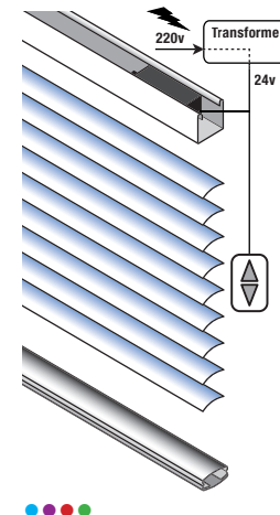
Electric Switch
